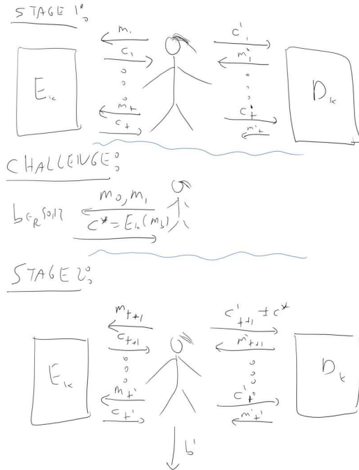
Figure 6.2: the CCA security game
