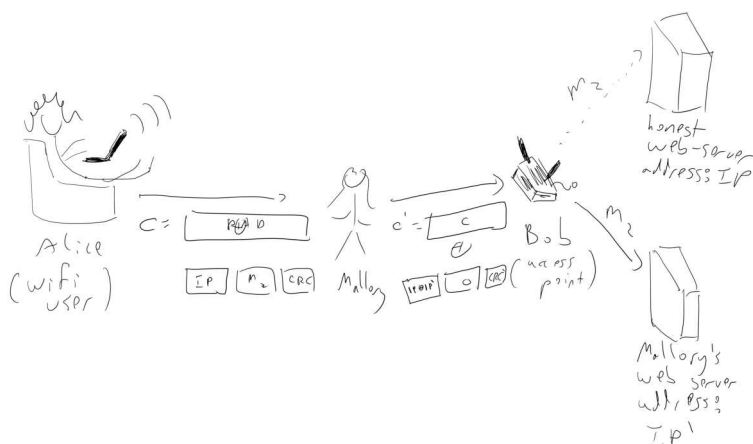
Figure 6.1: The attack on the WEP protocol allowing the adversary Mallory to read encrypted messages even when Alice uses a CPA secure encryption.
